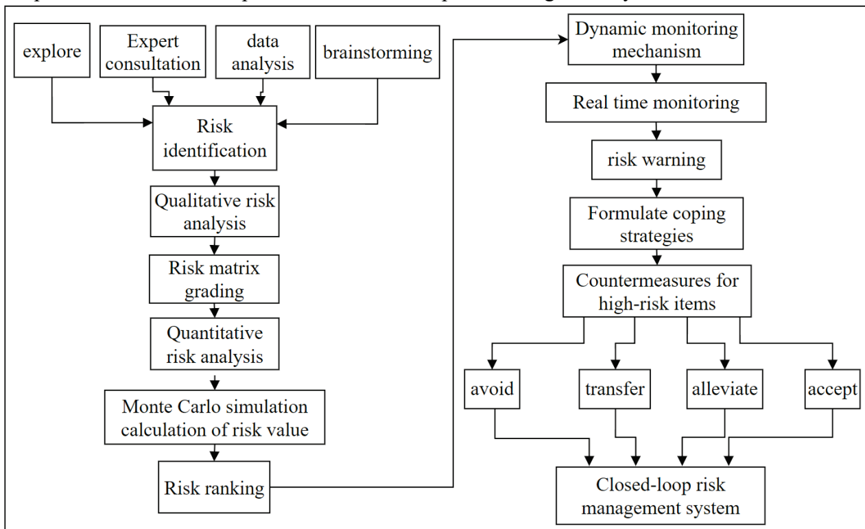
Figure 1 Risk assessment process of municipal road construction
